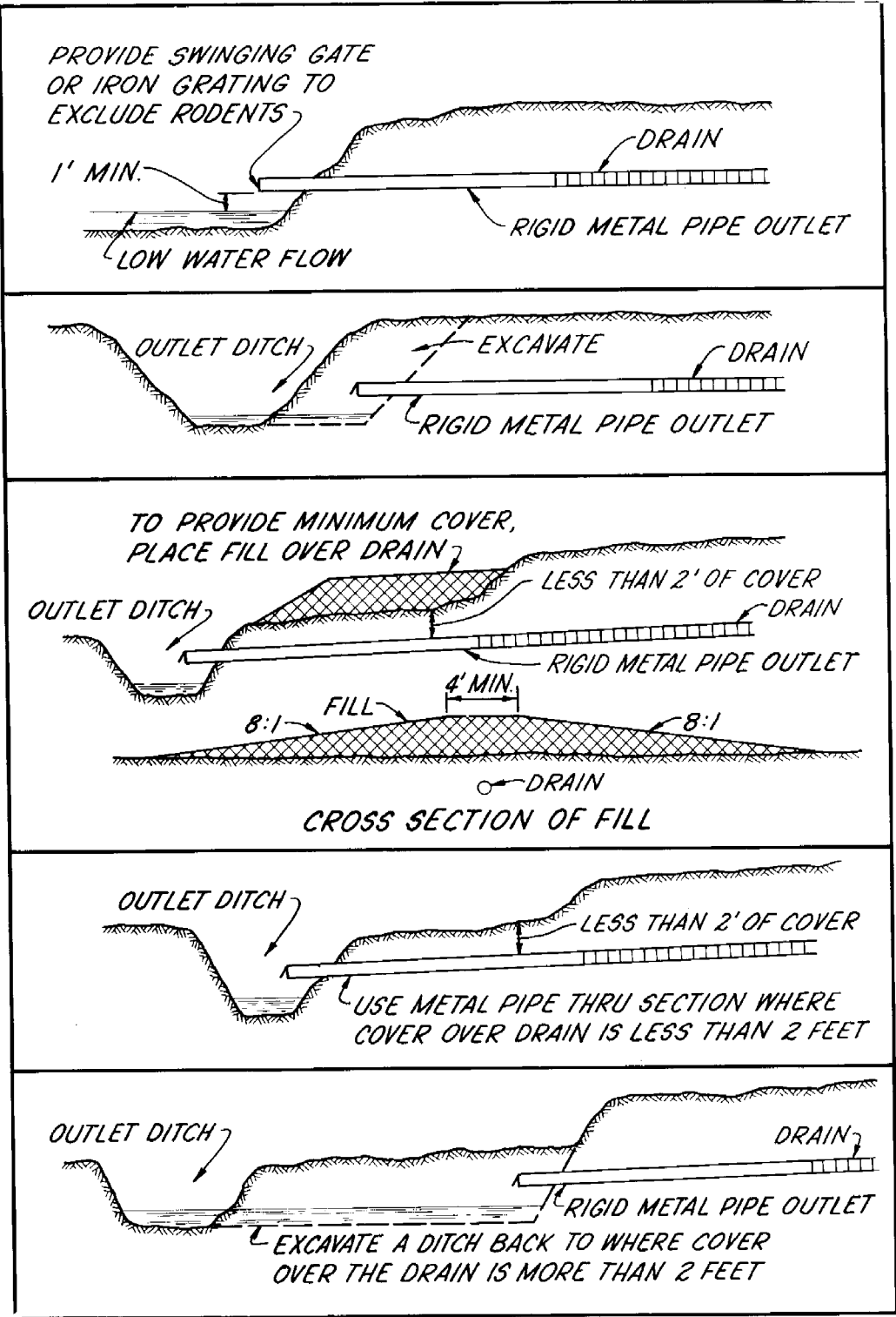
Figure 4-40, Drain outlets
