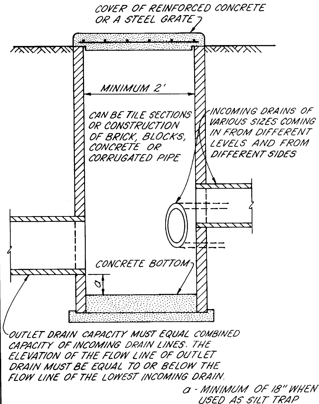
Figure 4-42, Junction box for drains
