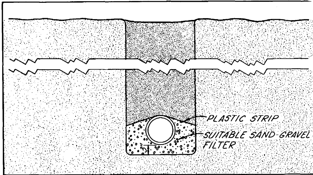
Figure 4-38, Filter installation
